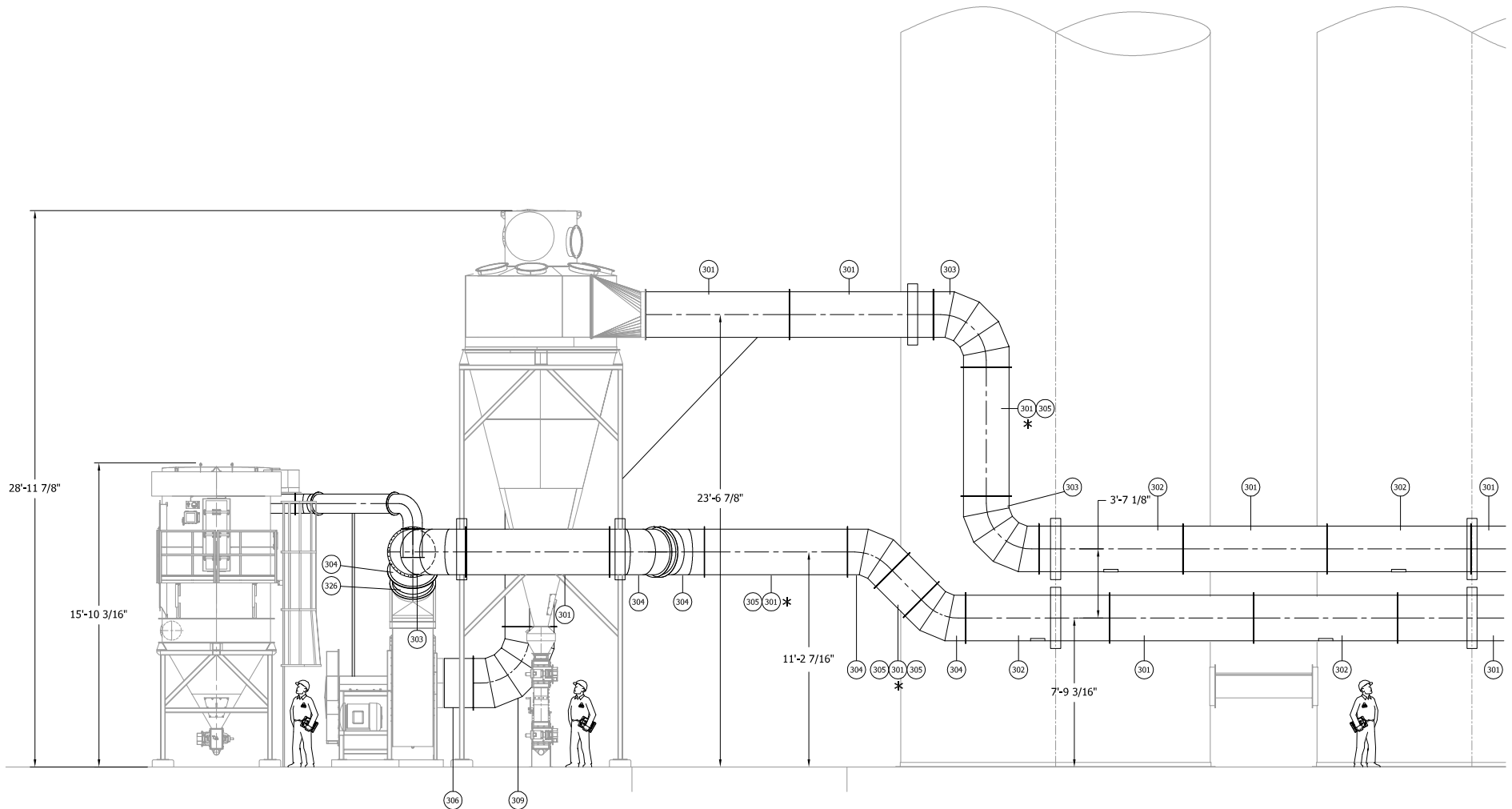
ELEVATION B-B LOOKING EAST
