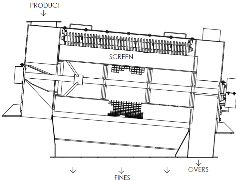
Figure 3 Flow Diagram
